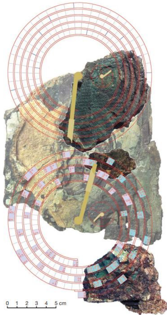
Figure 2. Depiction of reconstruction of the back dials of Antikythera,
