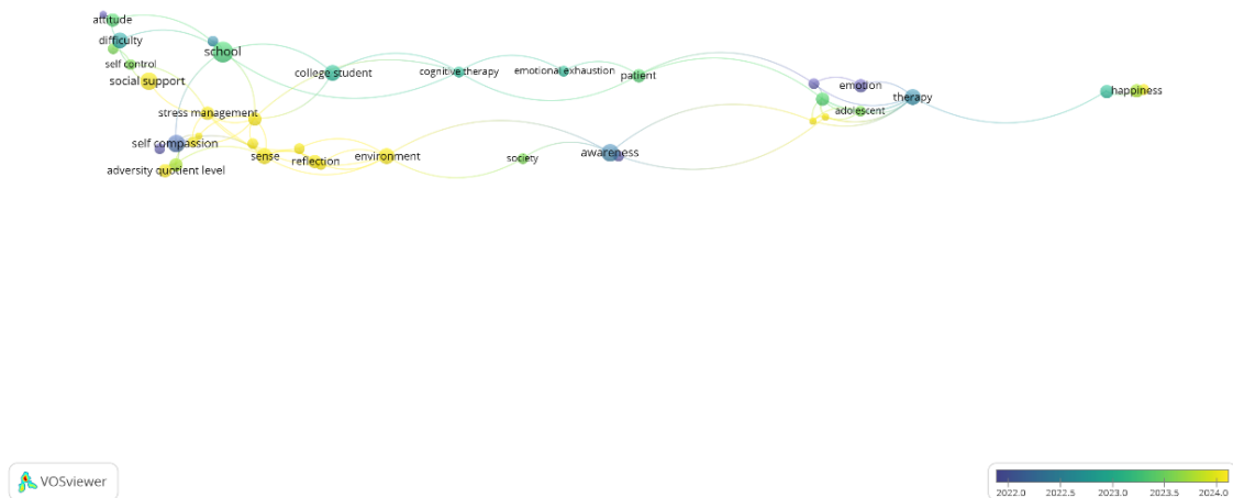
Figure 3. Overlay Visualization of Thematic Evolution in Mindfulness and Adversity Quotient Research (2020–2025)
