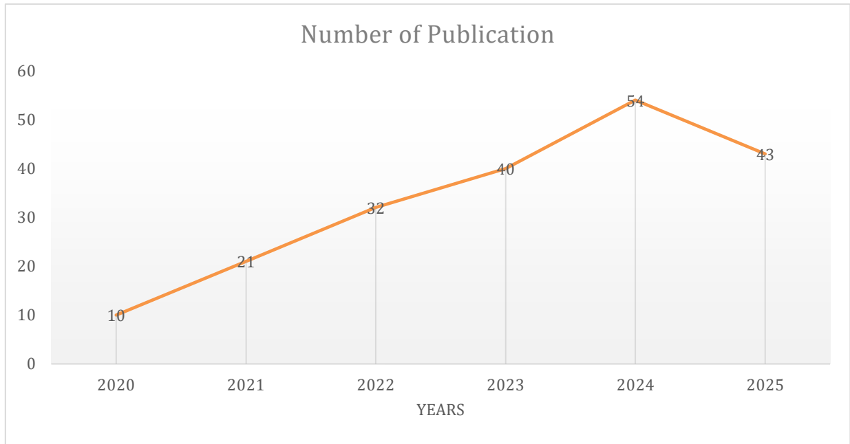
Figure 1. Annual report of publications
