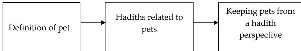
Chart 1. Thinking Framework
