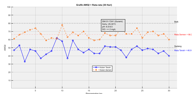
Figure 3. AWQI Calculation Results Generated Using MATLAB.
